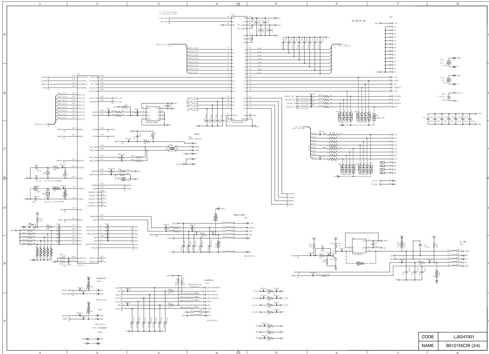
Appendix 5. Main PCB Circuit Diagram, HL-5170DN (2/4)
