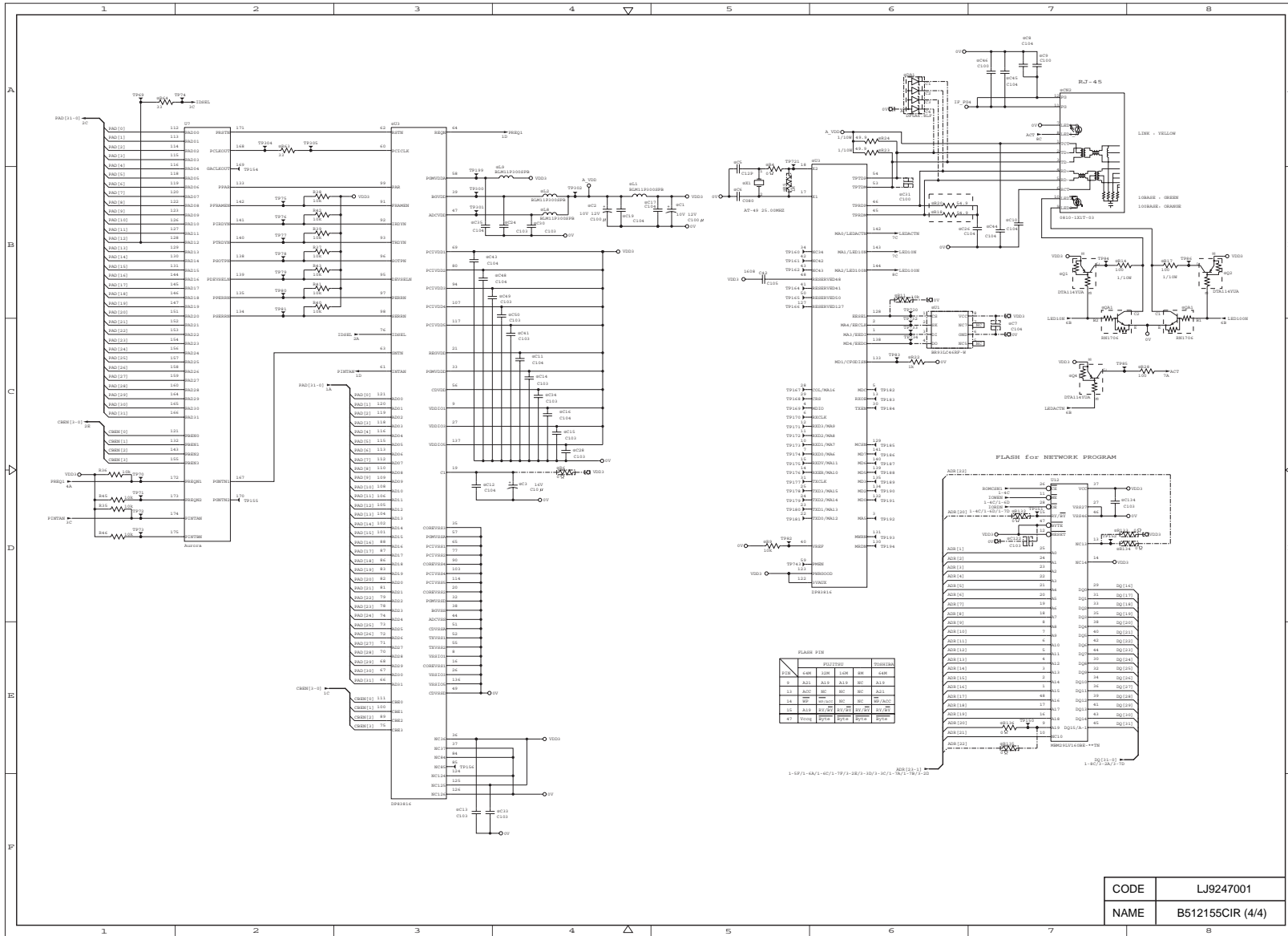
Appendix 7. Main PCB Circuit Diagram, HL-5170DN (4/4)
