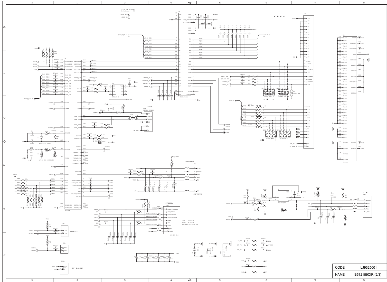
Appendix 2. Main PCB Circuit Diagram, HL-5130/5140/5150D (2/3)
