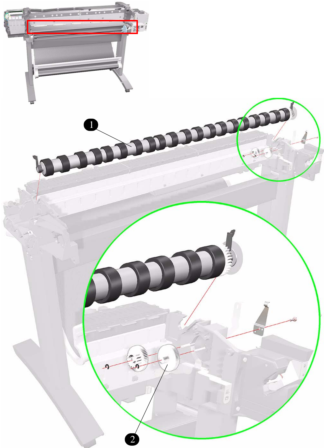
Figure 21: Drive Roller
