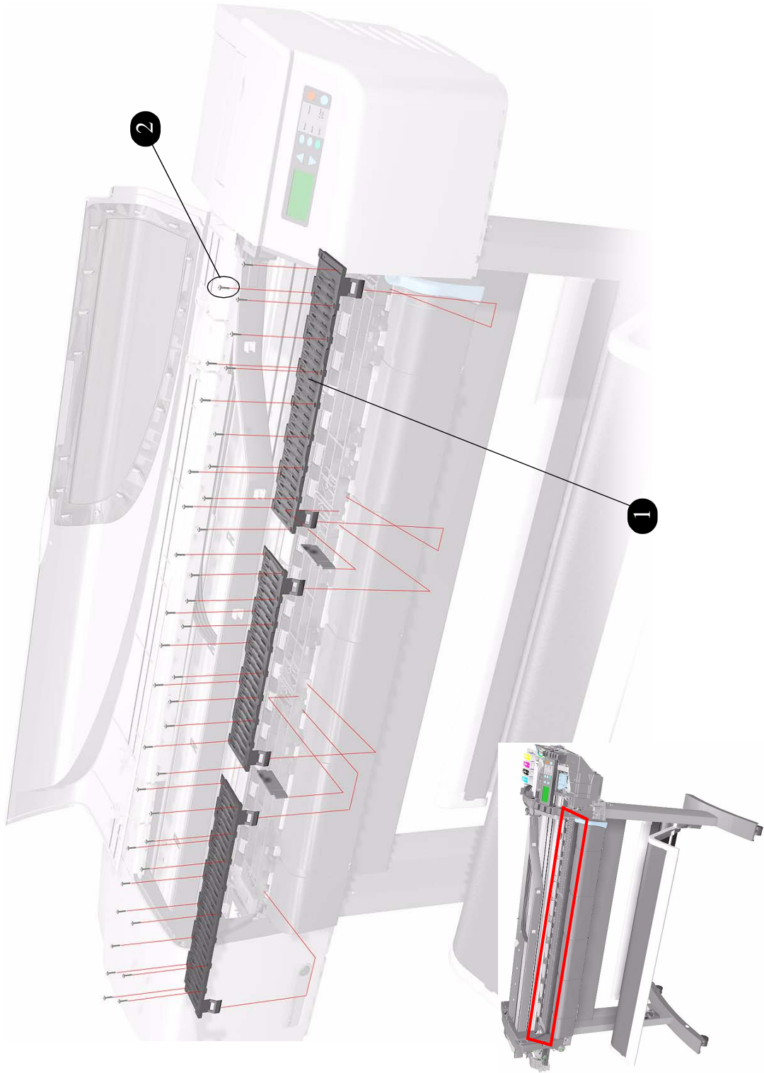
Figure 16: Print Platen Assembly
